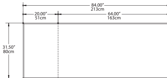
Plan View F2984VDL, F2984VDL-CE
