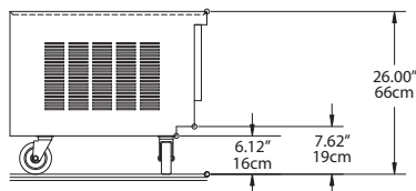
Left End View F2984VDL, F2984VDL-CE
